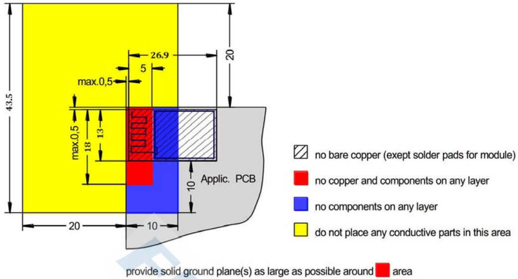
Figure 14: FSC-BT826E Restricted Area
